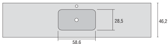
Cod. Vasca B224 cm 58,6 x 28,5 x 13 P Piletta esclusa Drain excluded
